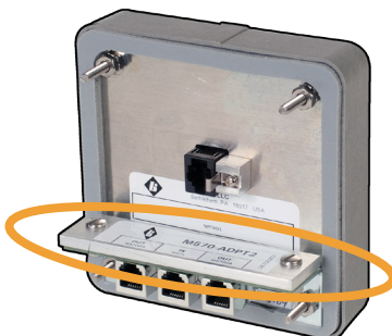
Dual display adapter shown mounted on M570DA display without panel
