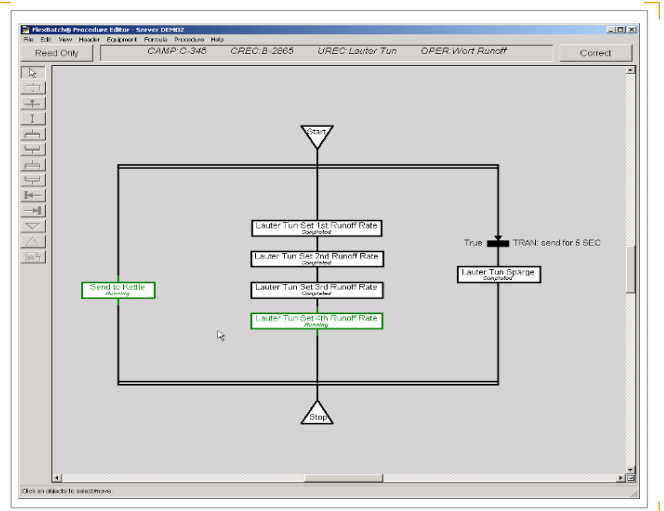
To simplify the creation, maintenance, and documentation of procedures, FlexBatch® uses a graphical procedure editor to create Procedure Charts™ that is based on the IEC 848 standard.
